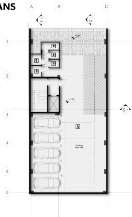
UNDER GROUND FLOOR PLAN
