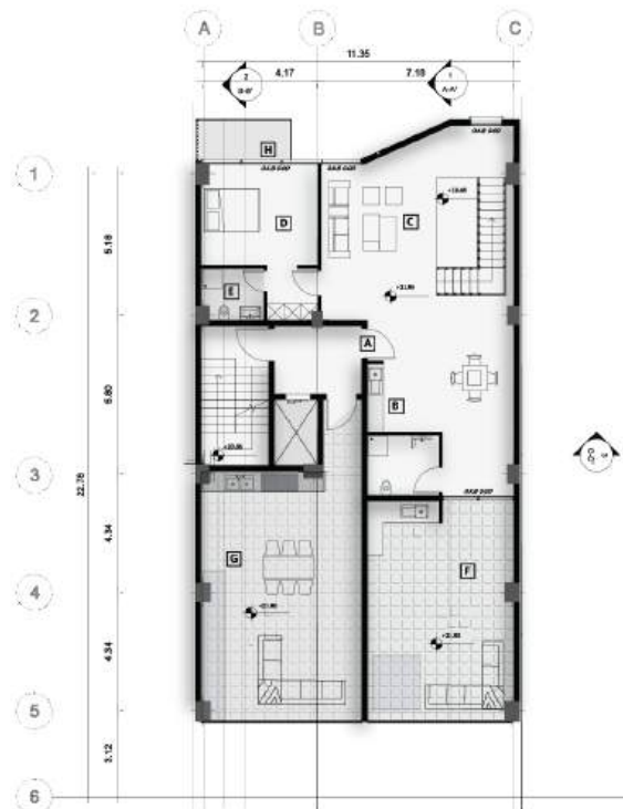
DUPLEX FIRST FLOOR PLAN
